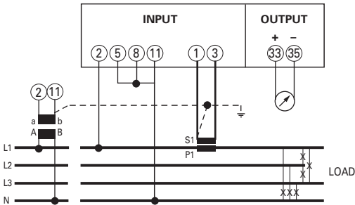
4-Leiter Drehstromnetz, gleich belastet Three-phase 4-wire, balanced load
