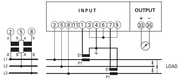
3-Leiter Drehstromnetz, ungleich belastet ARON Three-phase 3-wire, unbalanced load ARON
